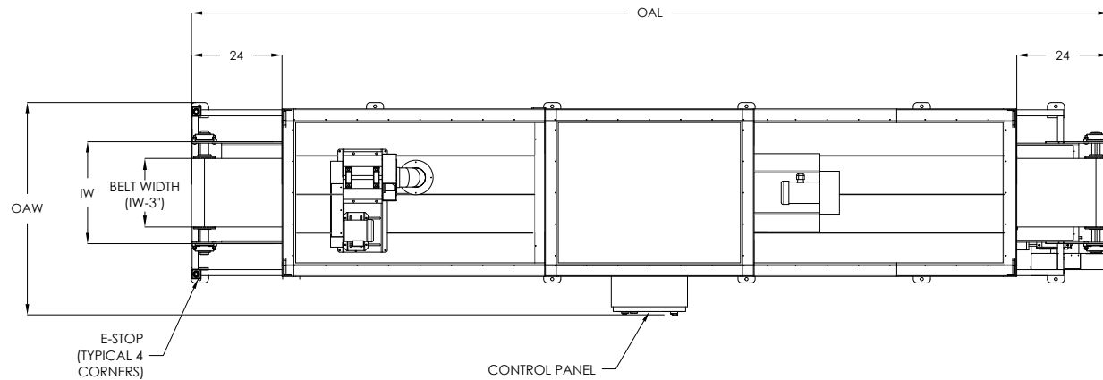
PLAN VIEW
