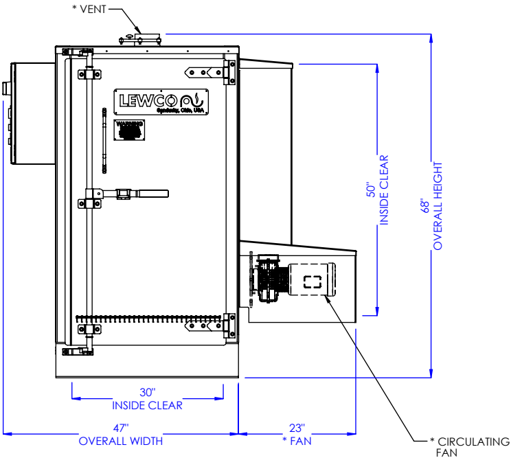
FRONT ELEVATION
