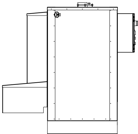
REAR ELEVATION
