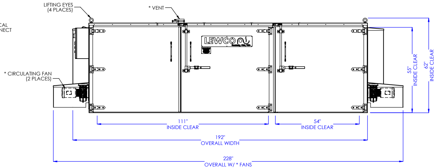
FRONT ELEVATION
