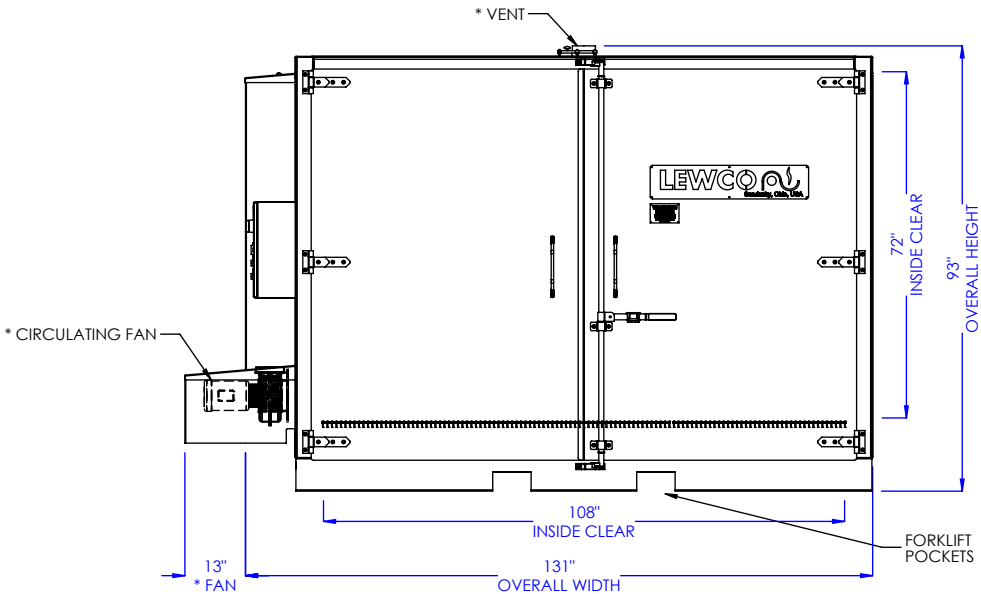
FRONT ELEVATION
