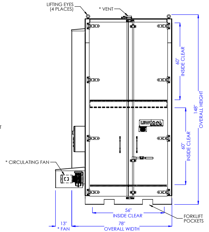
FRONT ELEVATION
