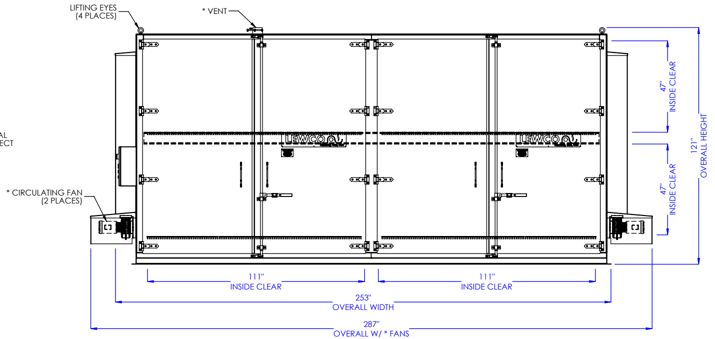
FRONT ELEVATION
