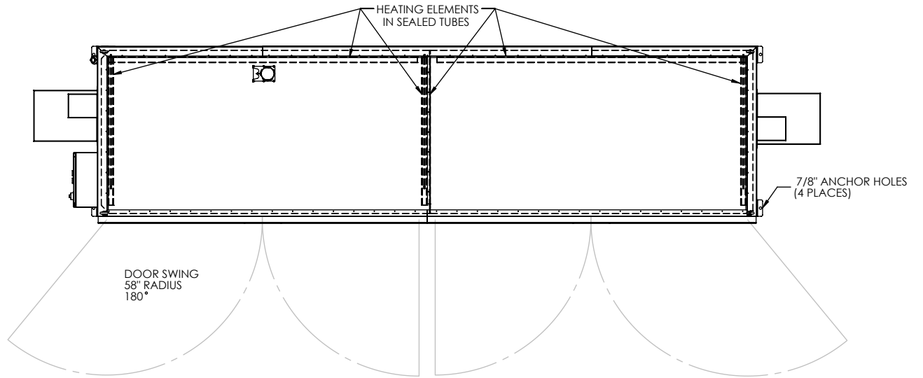
PLAN VIEW
