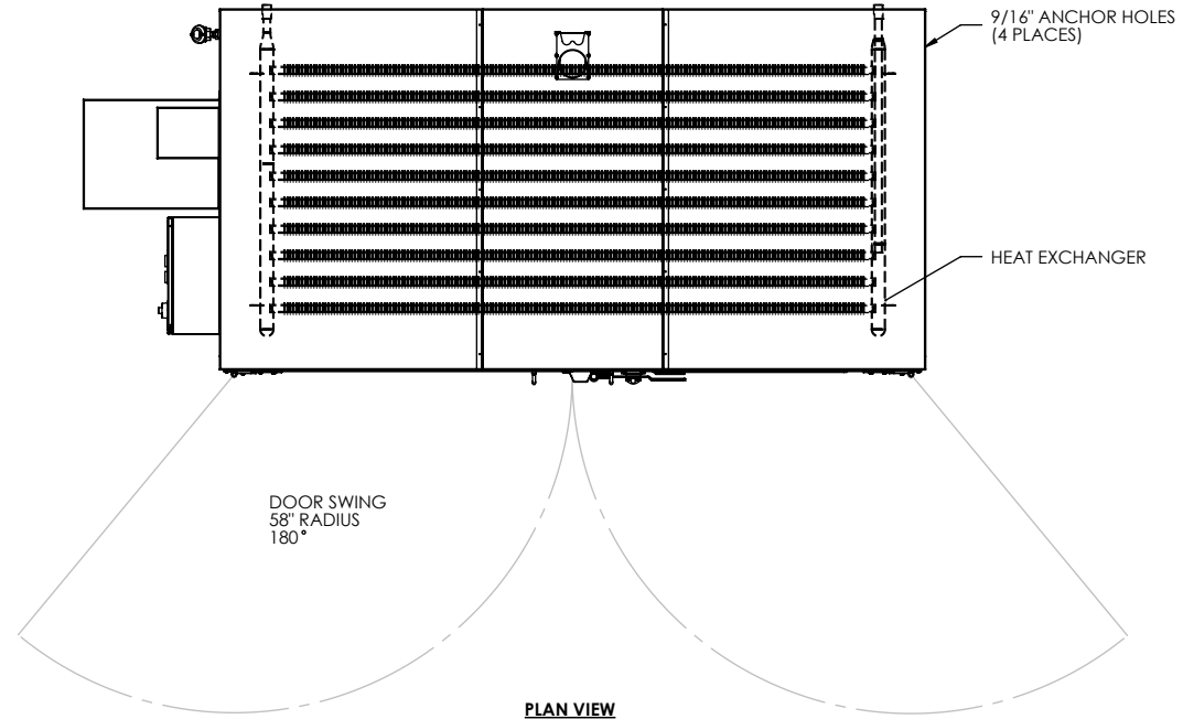
PLAN VIEW
