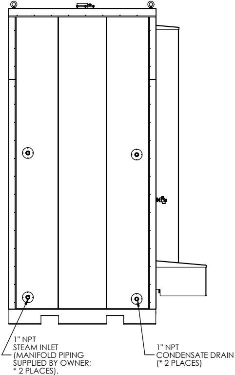
REAR ELEVATION
