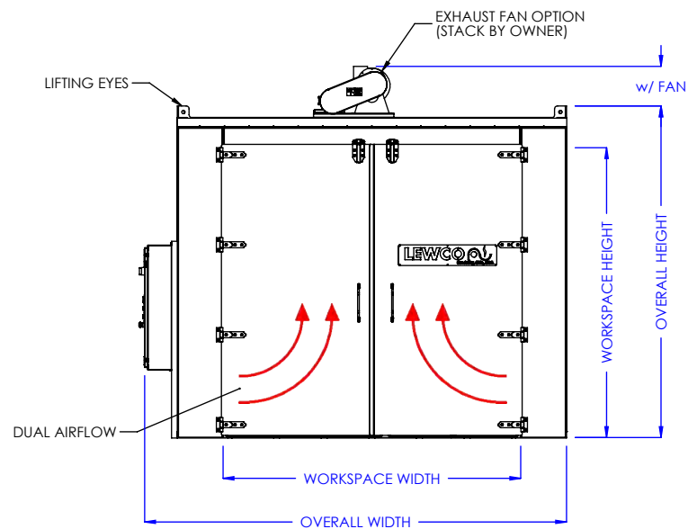
FRONT ELEVATION
