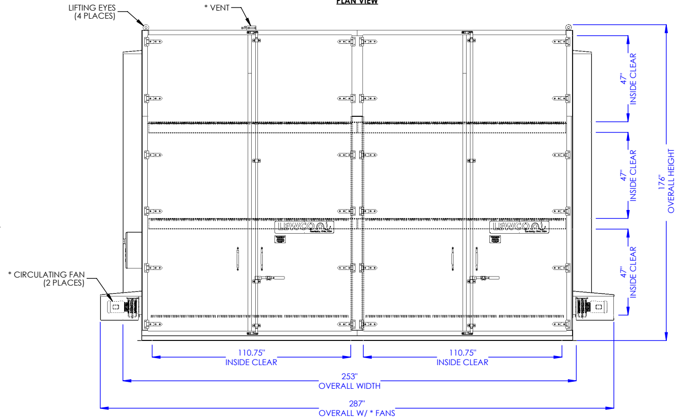
FRONT ELEVATION
