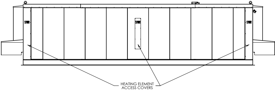
REAR ELEVATION
