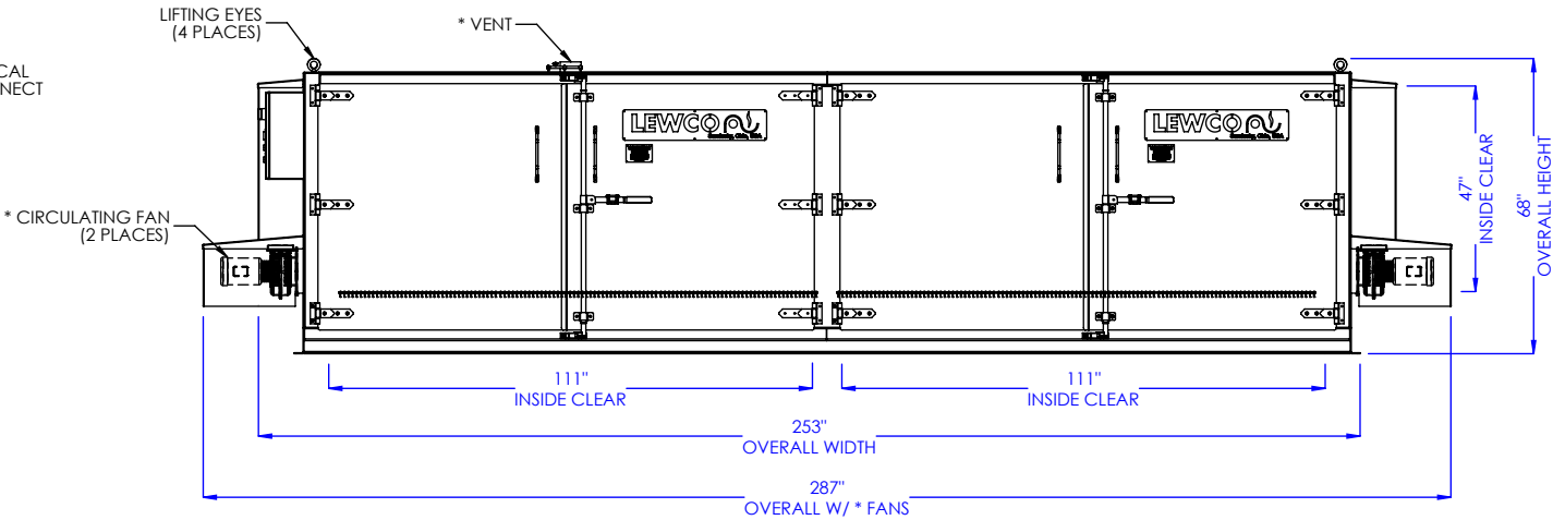
FRONT ELEVATION
