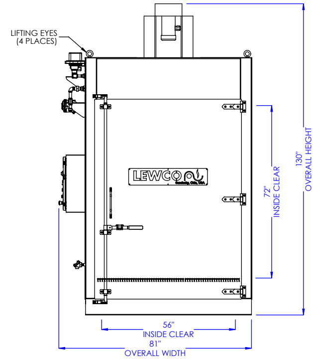
FRONT ELEVATION
