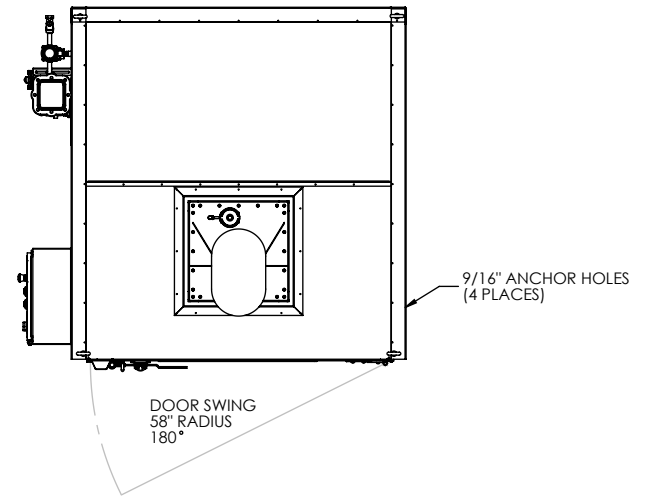
PLAN VIEW
