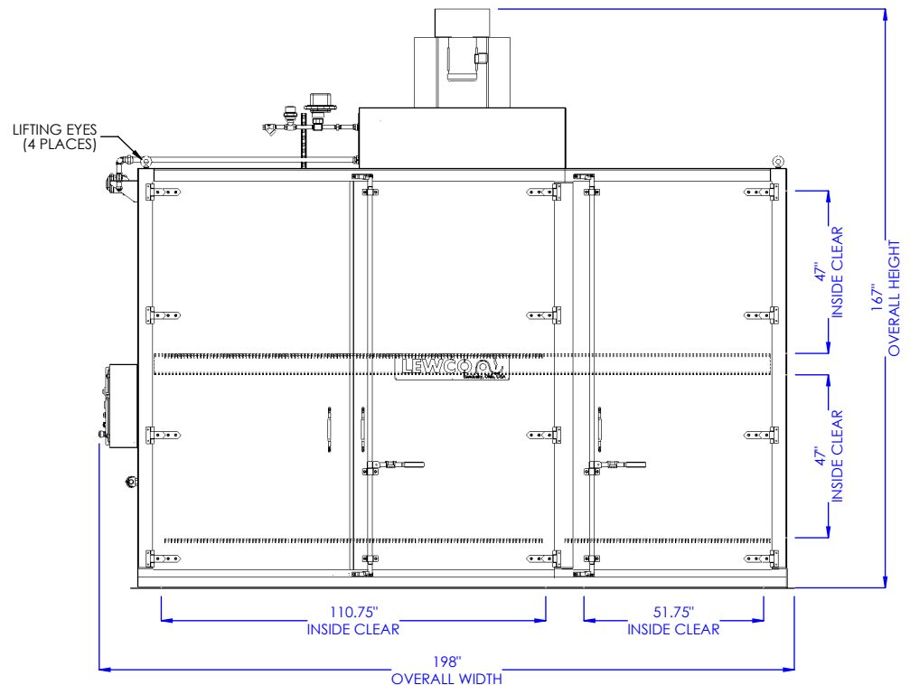
FRONT ELEVATION
