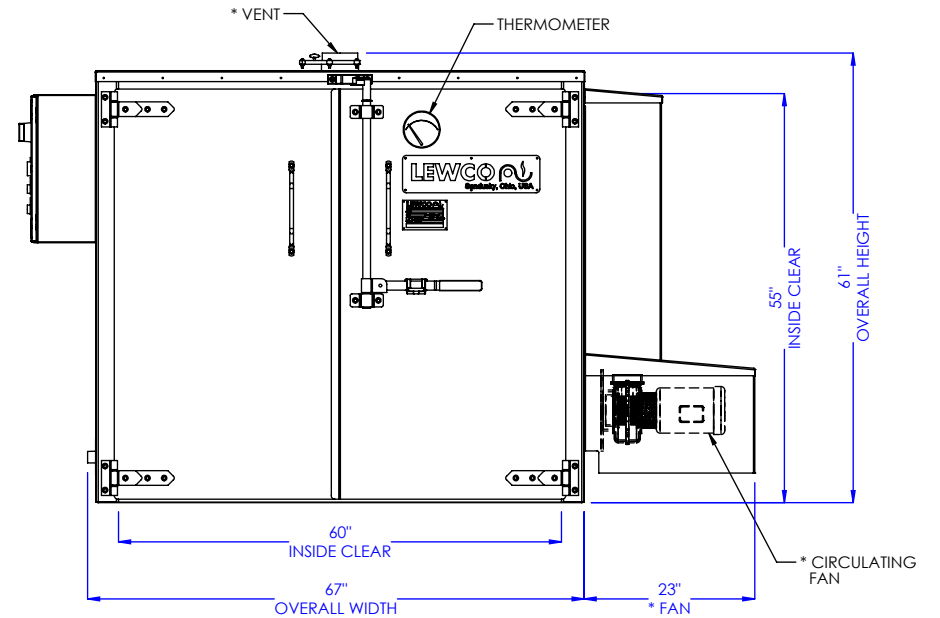
FRONT ELEVATION
