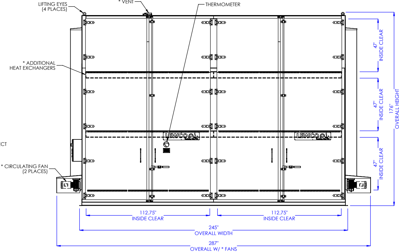
FRONT ELEVATION
