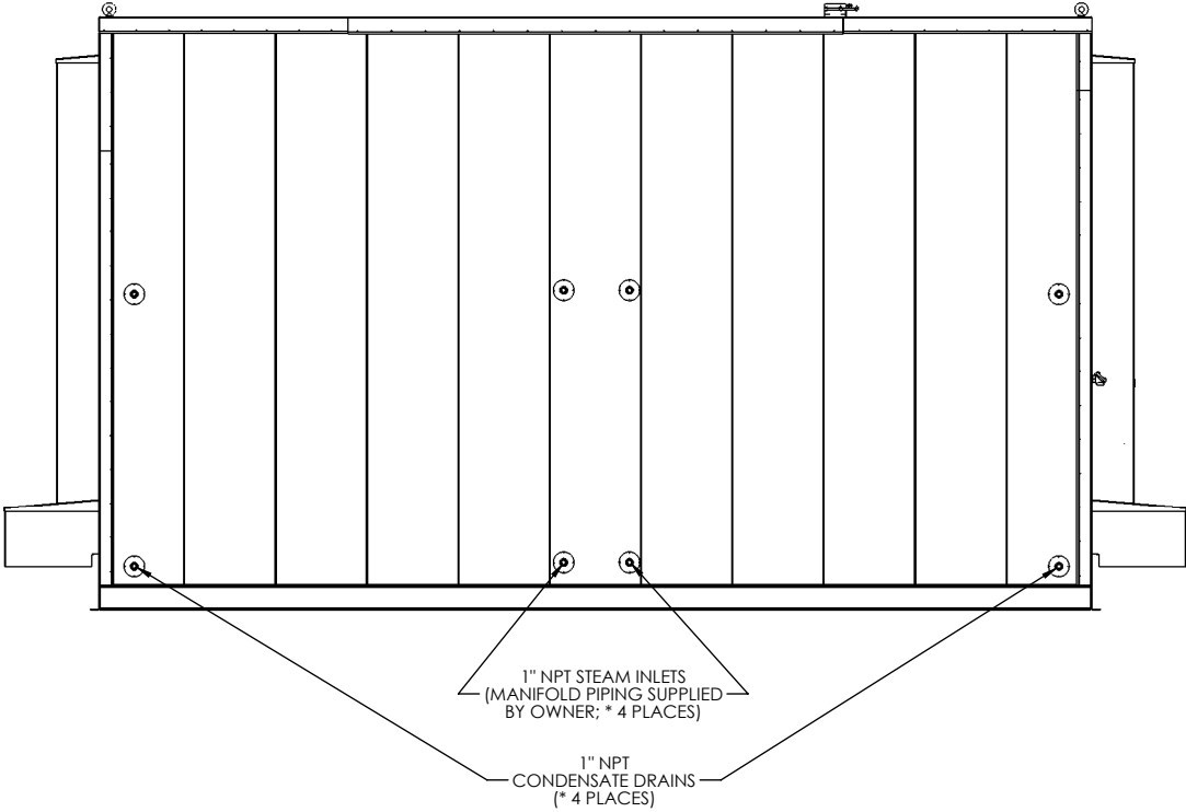
REAR ELEVATION
