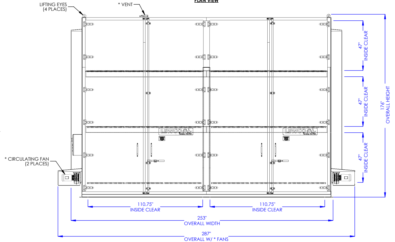
FRONT ELEVATION
