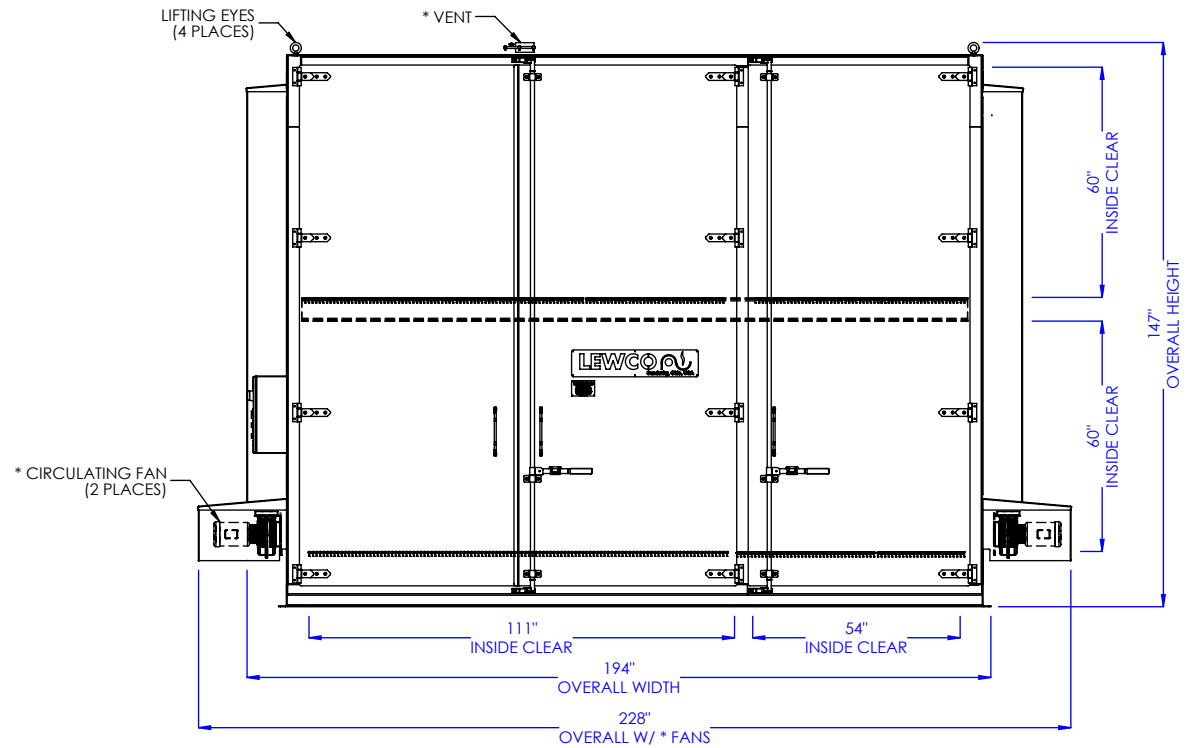
FRONT ELEVATION
