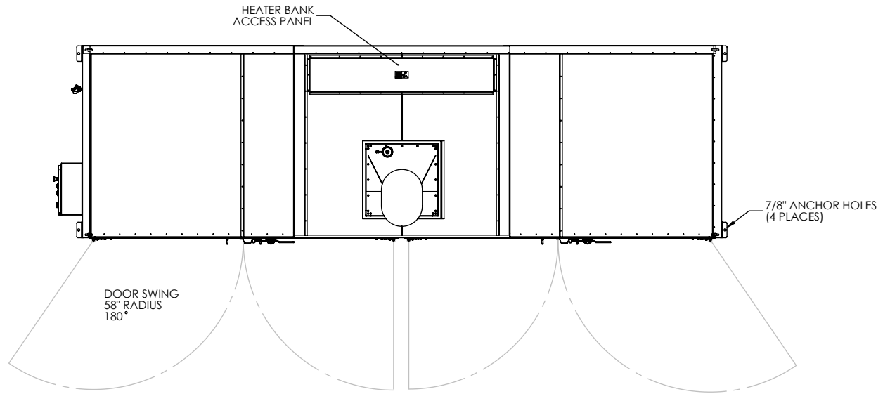
PLAN VIEW
