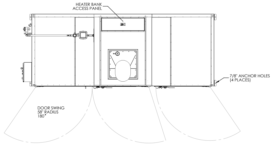
PLAN VIEW
