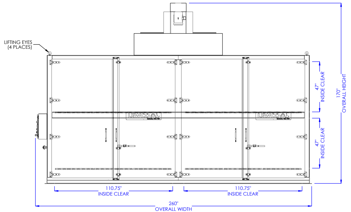
FRONT ELEVATION
