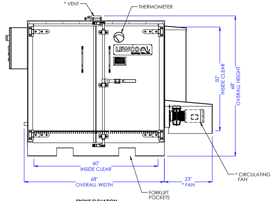
FRONT ELEVATION
