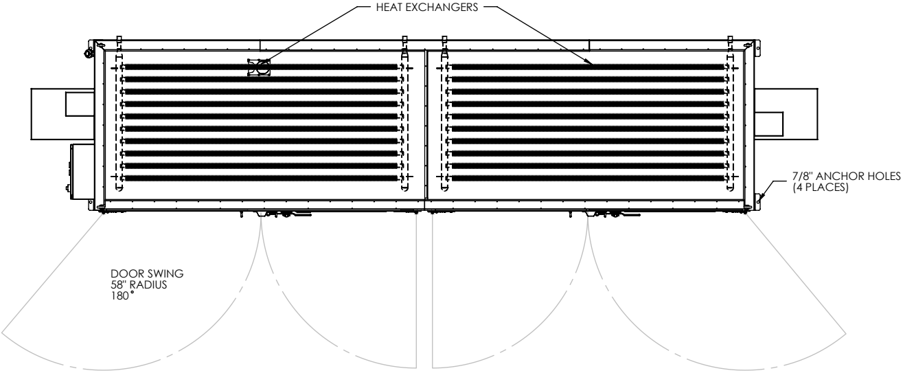
PLAN VIEW
