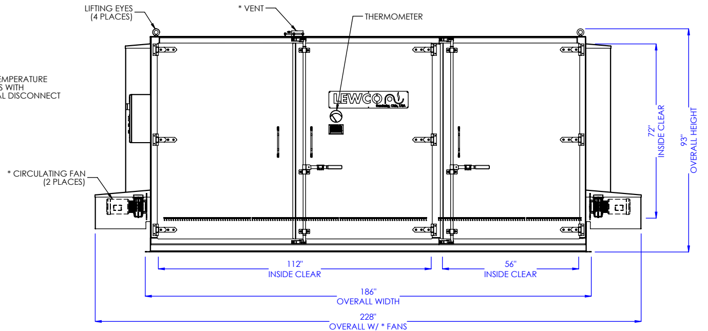
FRONT ELEVATION
