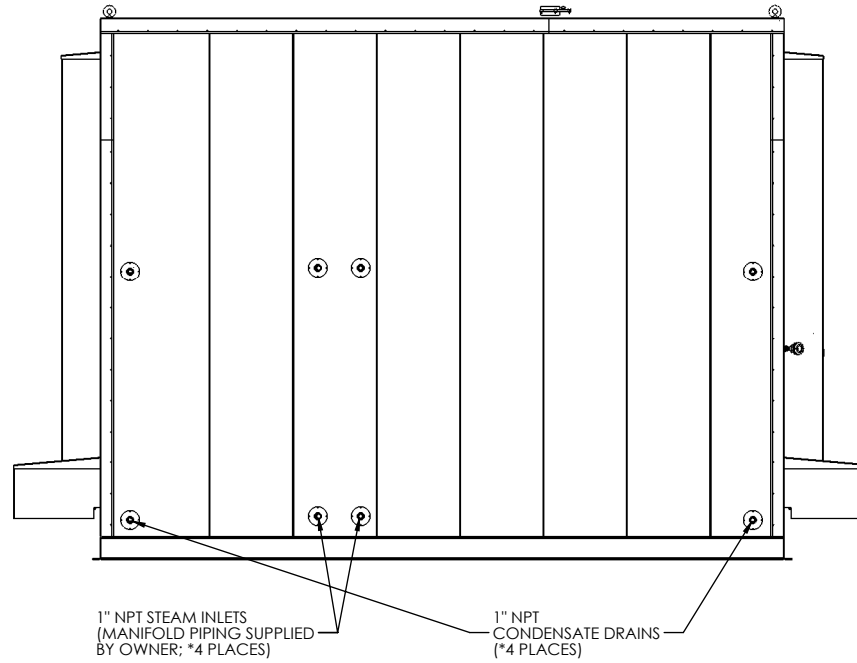
REAR ELEVATION
