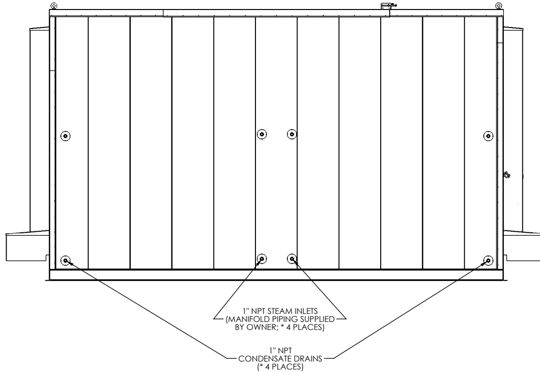
REAR ELEVATION
