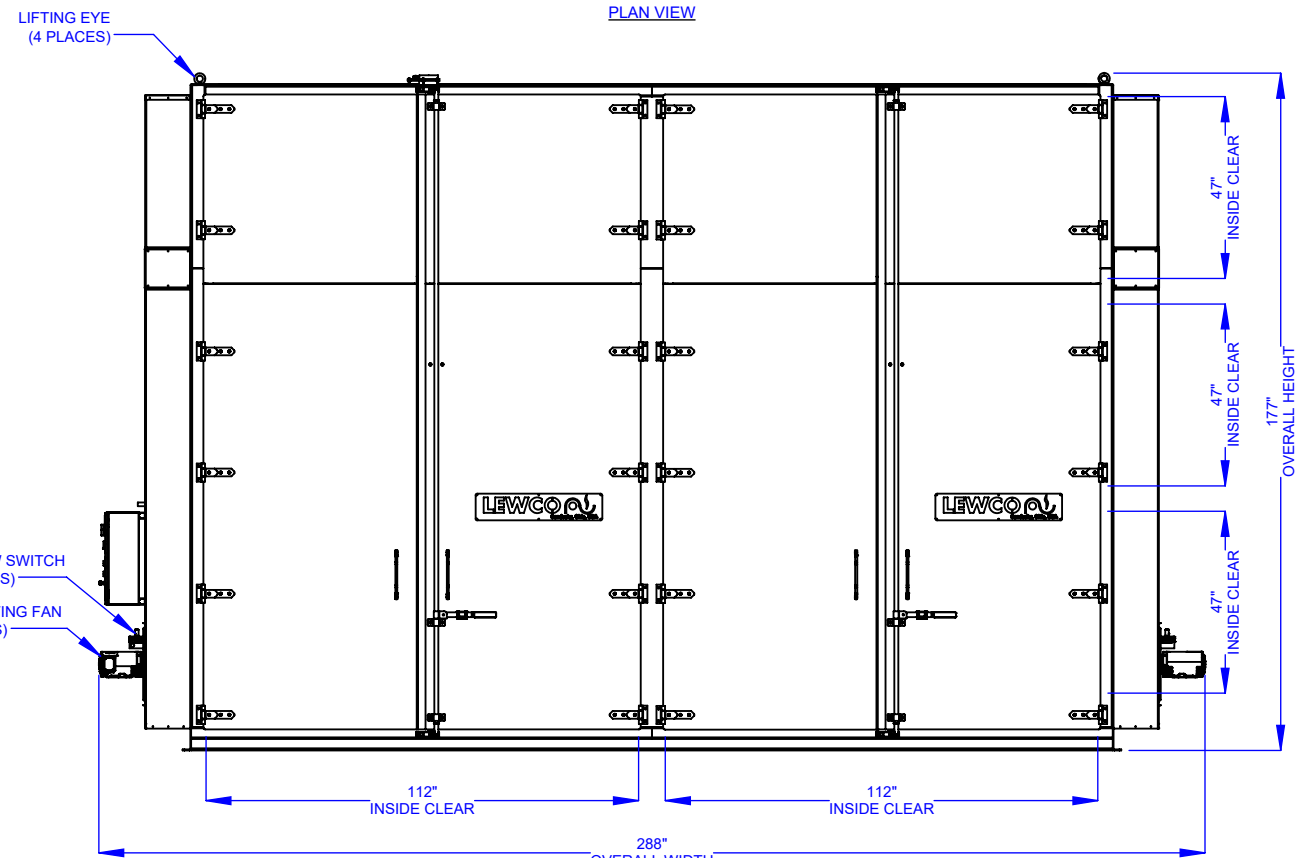
FRONT ELEVATION
