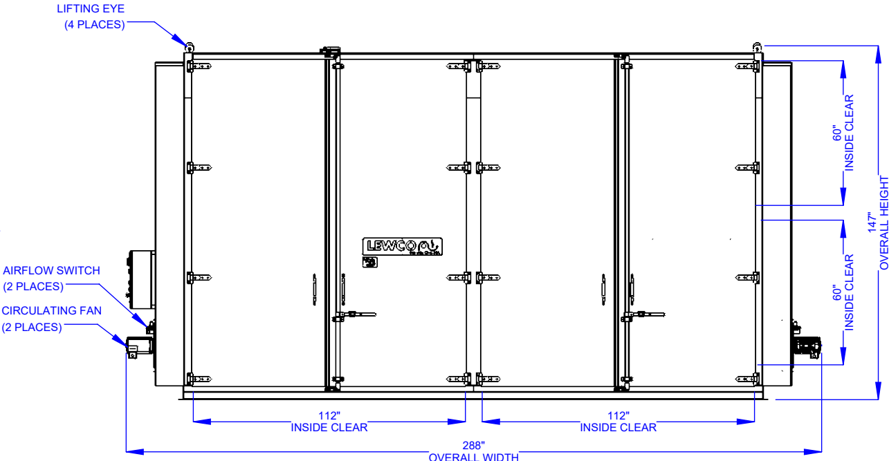
FRONT ELEVATION
